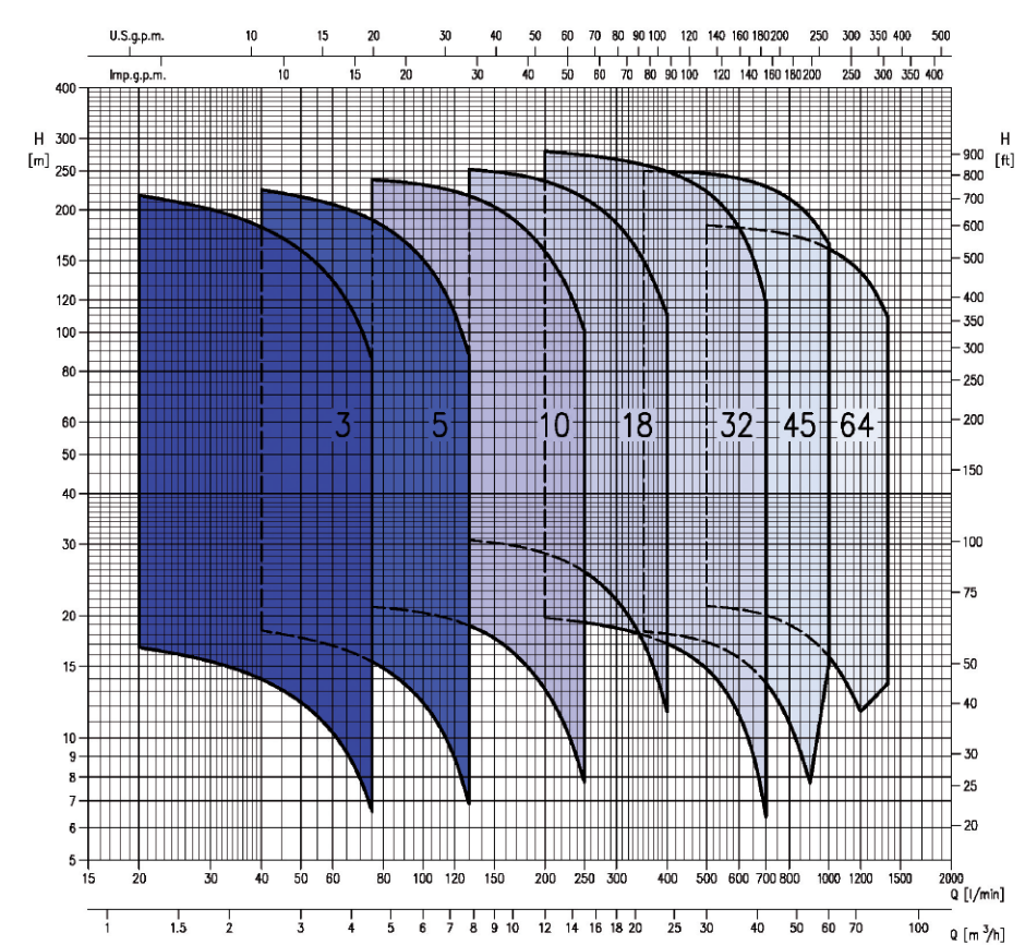
PERFORMANCE RANGE
